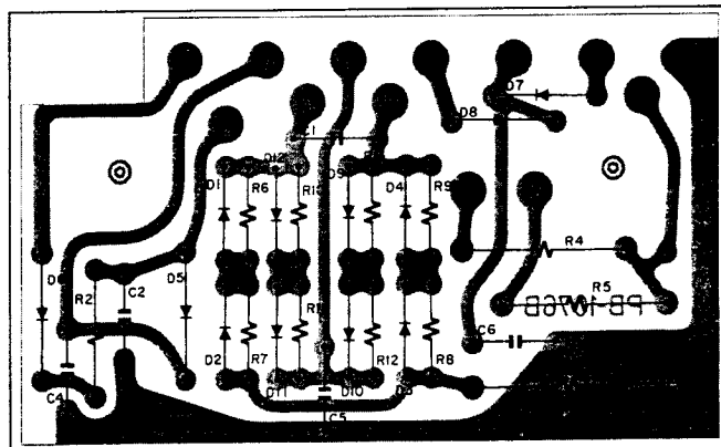
Viewed From Component Side
