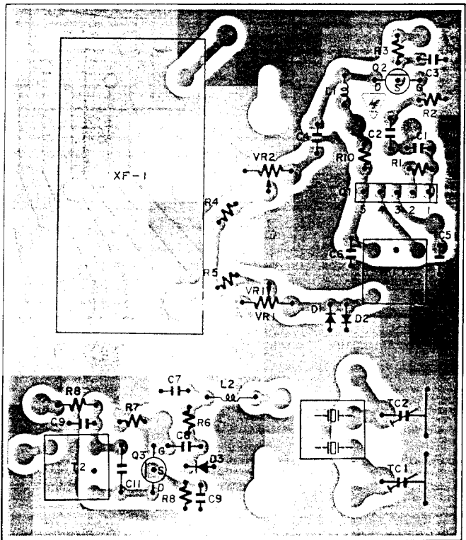
Viewed From Solder Side
