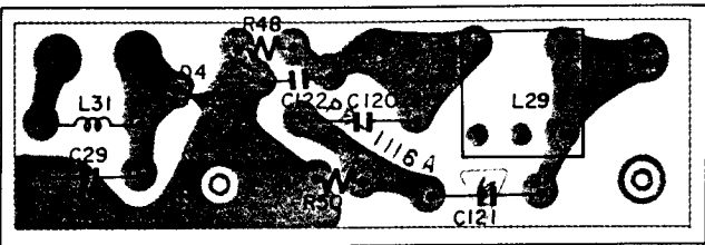
Viewed From Solder Side
