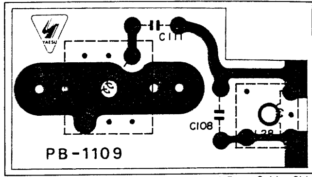
Viewed From Solder Side
