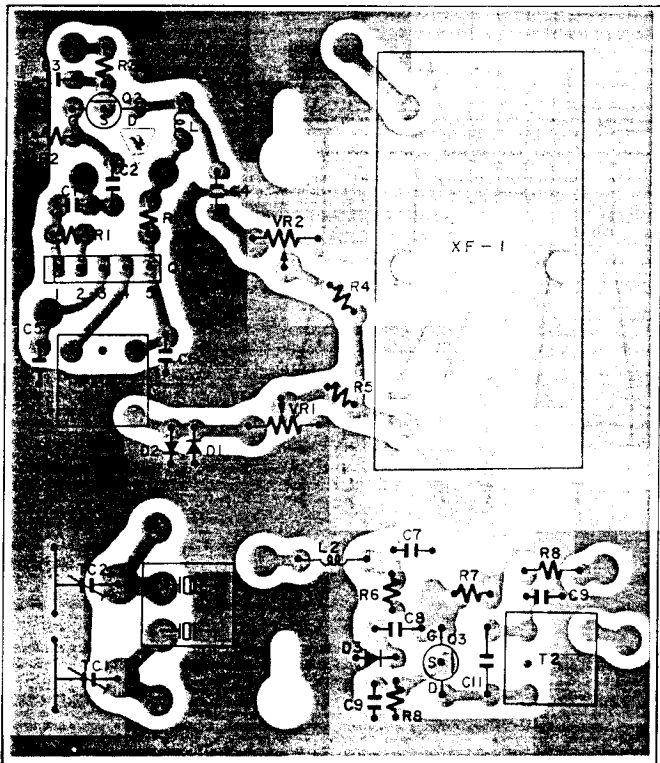
Viewed From Component Side
