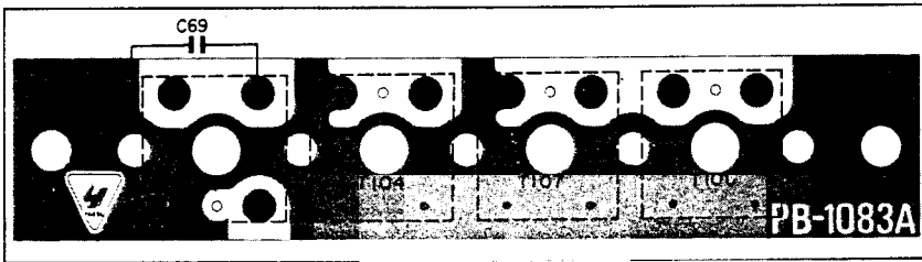
Viewed From Solder Side
